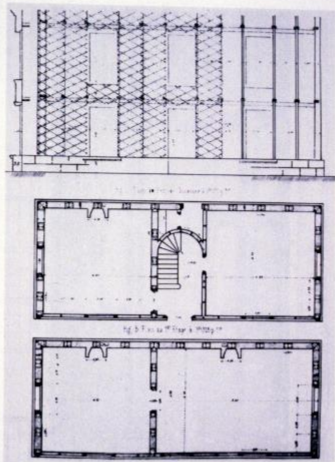
Plate 59. Lacroix system of framing with iron and cement or concrete ( Nouvelle annales de la construction , X, January, 1864, pl. 7)
